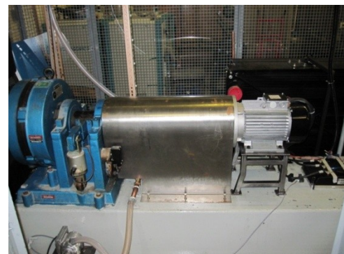
Fig. 2. Dynamometer hardware
