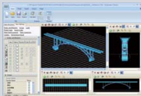
▲Engineer's Studio®
